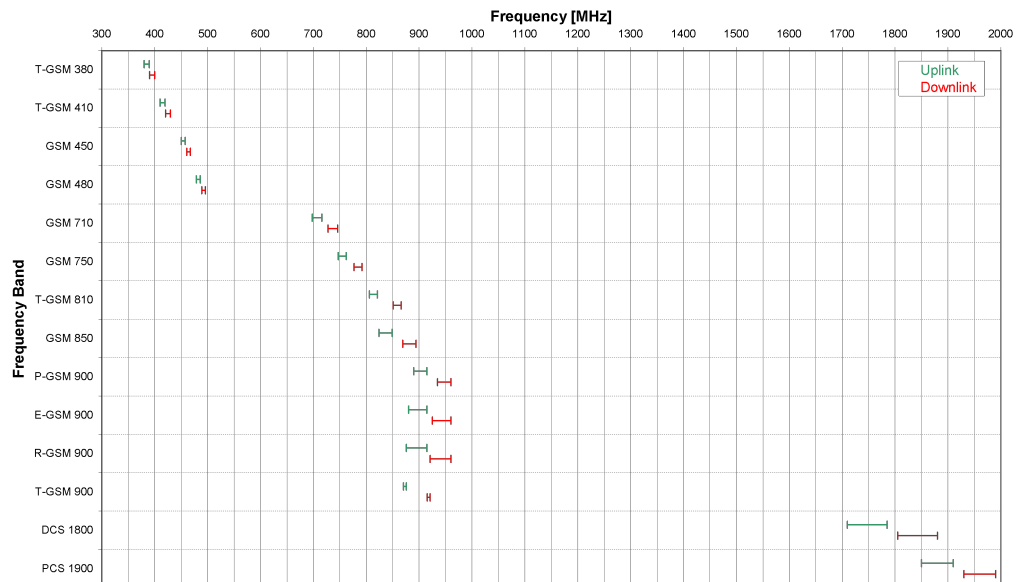
Fig. 3-19: The frequencies specified in the GSM standard
