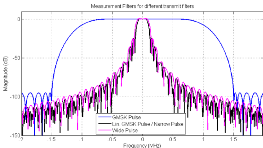
Fig. 3-28: Magnitude Responses of Measurement Filters for Demodulation Measurements
