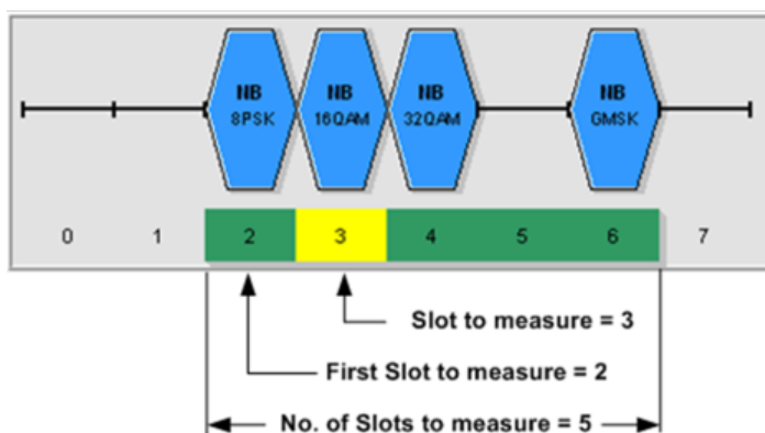
Fig. 3-23: Concept of "First Slot to measure", "Number of Slots to measure" and "Slot to Measure"
